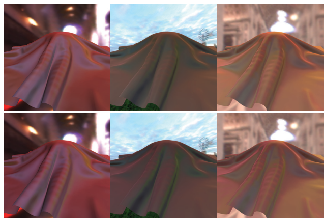
Fig. 14 Rendering of the fitted 3-axial BRDF in different illumination environments. The first row features the reference BRDF while the second row shows its fitting by our model.
