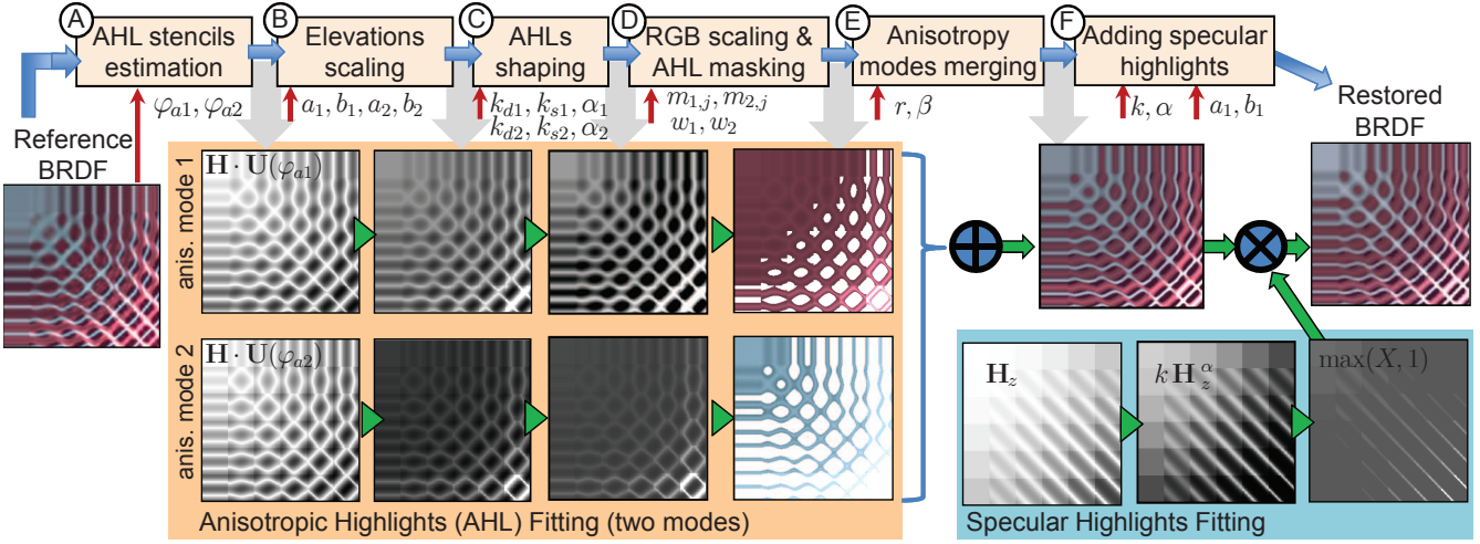
Fig. 4 Overall scheme of the proposed BRDF model.
