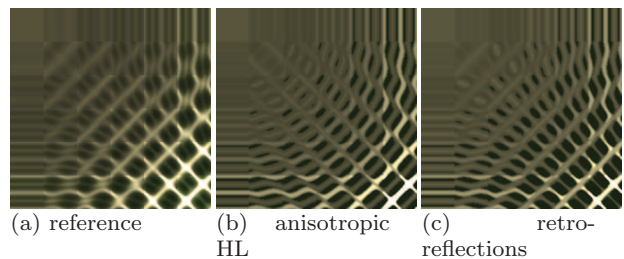
Fig. 11 Extension to retro-reflection highlights modeling: (a) reference BRDF, reconstructed BRDF (b) with anisotropic highlights, (c) with retro-reflective highlights.
