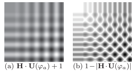
Fig. 6 Highlights stencil: predicting of anisotropic highlight location (b) using a dot-product of half-way direction \mathbf{H} and the detected direction of anisotropy \mathbf{U} = [\sin \varphi_a, \cos \varphi_a, 0] , for \varphi_a = 0^\circ .
