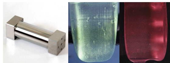
Figure 2: Cylindrical film applicator (left) and two tested pigments applied on a plastic material with black glossy basecoat (middle, right).
